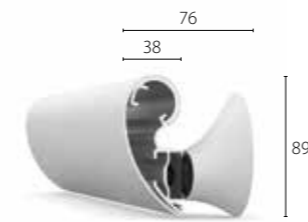
HRB-35N
