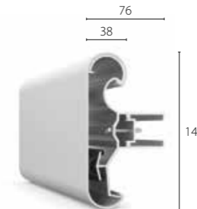
HRB-4CAL
