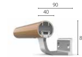
HRE-6-A80
