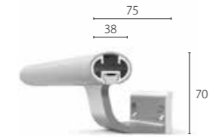
HRO-6-A80
