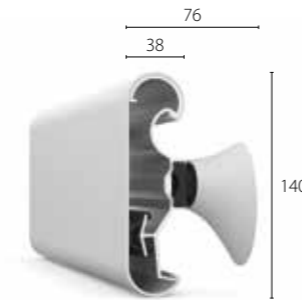
HRB-4C
