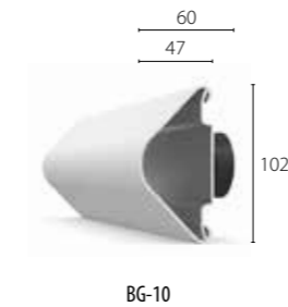
BG-10
